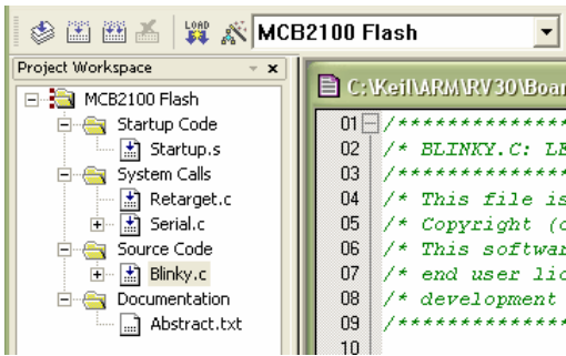
FIGURE 6 μVision3 Project Workspace window showing OPENED MCB2100 Blinky Flash application.
