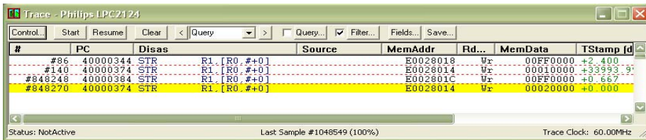
FIGURE 53 Filtered trace showing only read and write to the IO ports operations.
