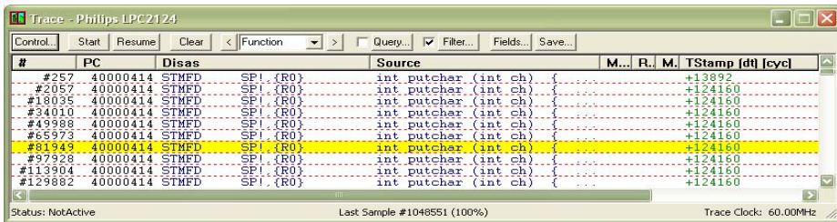
FIGURE 49 Filtered trace showing calls to only one function.
