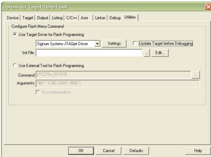
FIGURE 19 Selecting the Signum JTAGjet Driver as the flasher for the Hello Flash target of the HelloR project.
